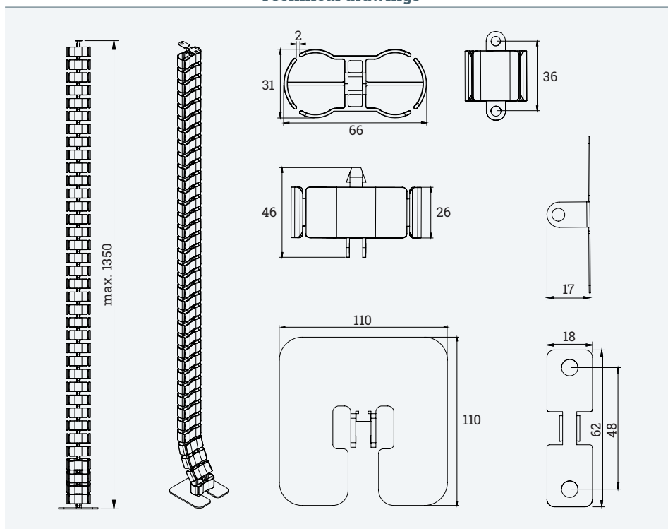
Optional magnetic top connector
