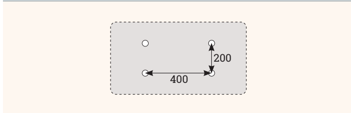
Position: Drilling holes in the AKUSTIX element
