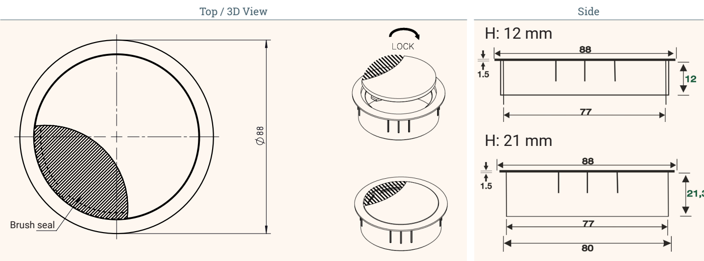
Technical Drawings
