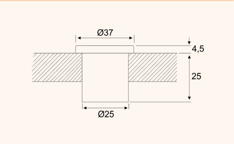
Technical Drawing
