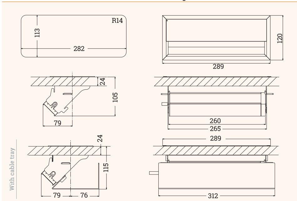
Technical Drawings
