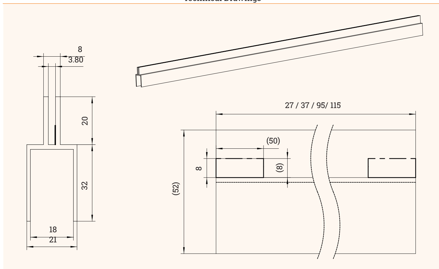
Technical Drawings
